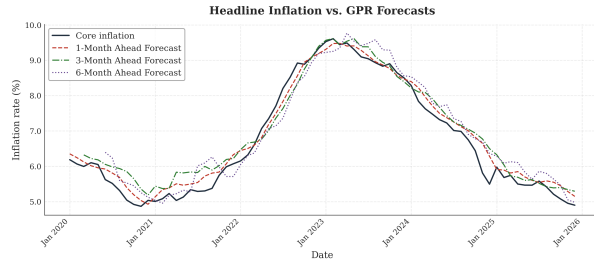
(e) GPR
