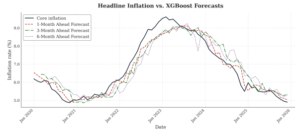
(g) XGBoost
