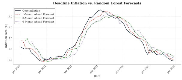
(f) Random Forest
